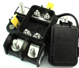
LITTELFUSE 600A, 2 Pole MEGA Fuse Sealed HPDM Item #46319
